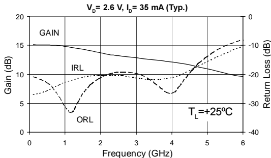
Gain & Return Loss vs. Frequency
